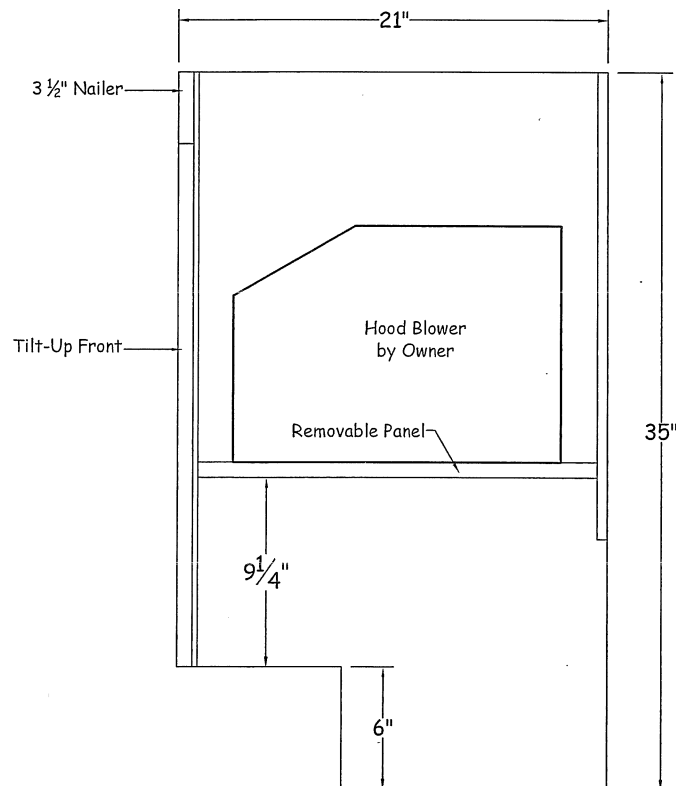
SECTION VIEW
